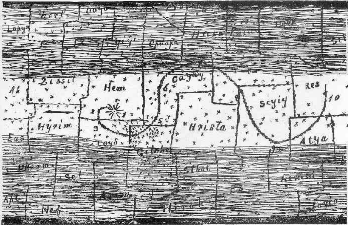
Plate 38.—ANOAD.
