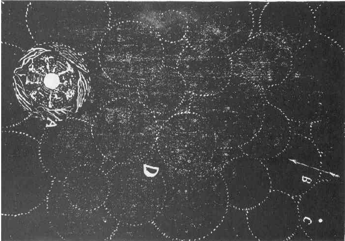
Plate 41. — PHOTOSPHERES.
