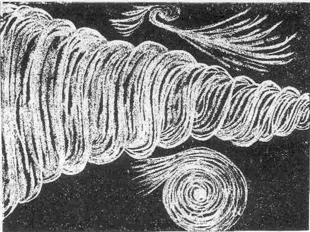
Plate 26.—SECONDARY VORTEX.
