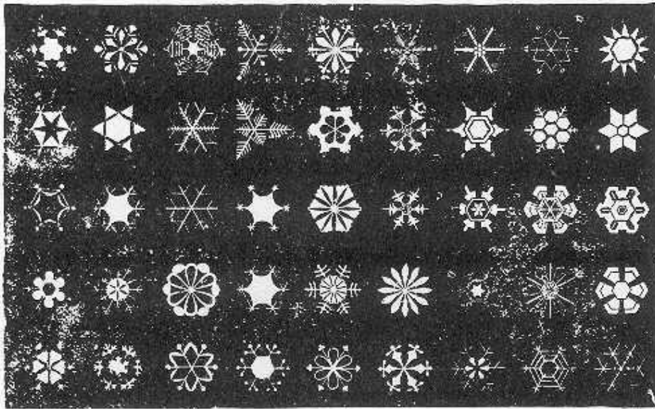
Plate 44.—SNOW-FLAKES.
