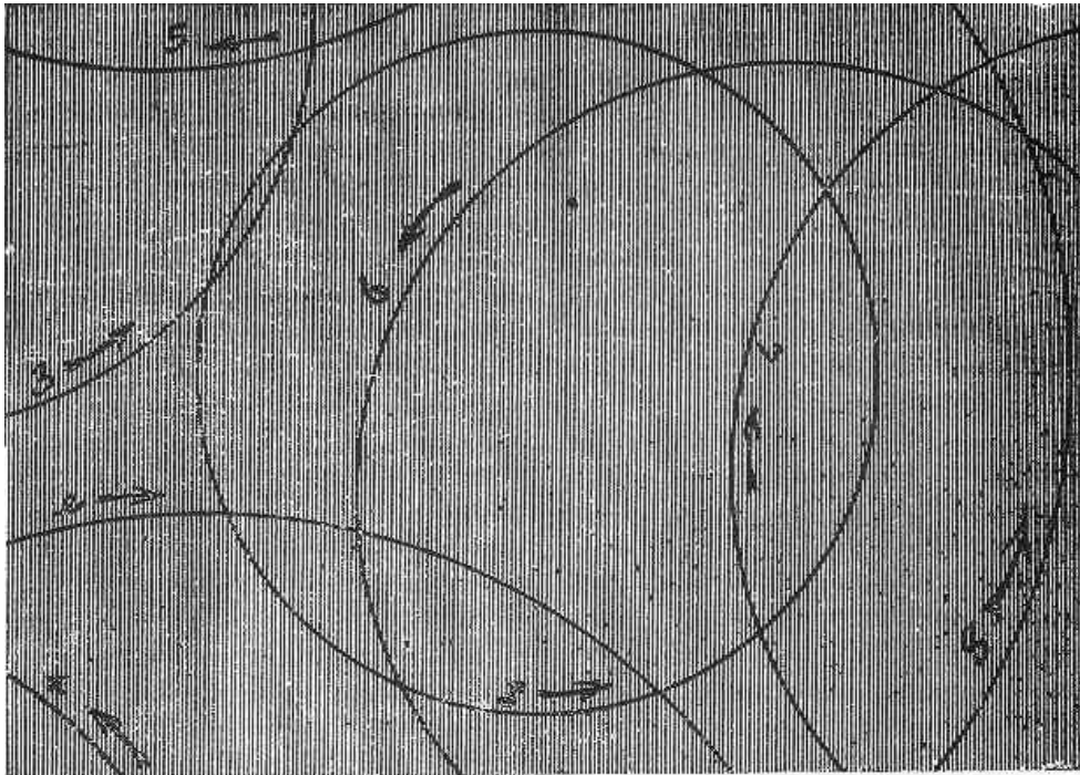
Plate 42.—SERPENT'S ORBIT.
