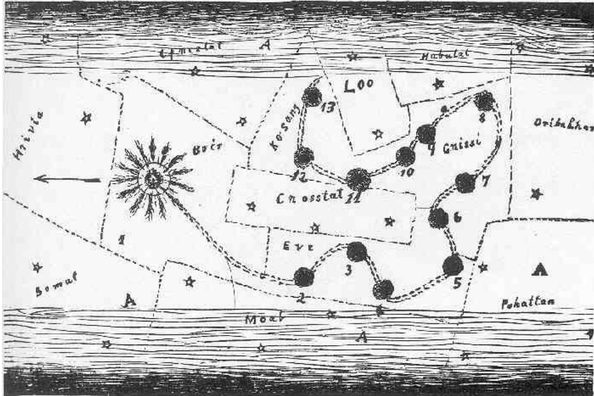
Plate 40.—SHAMMAEL.
